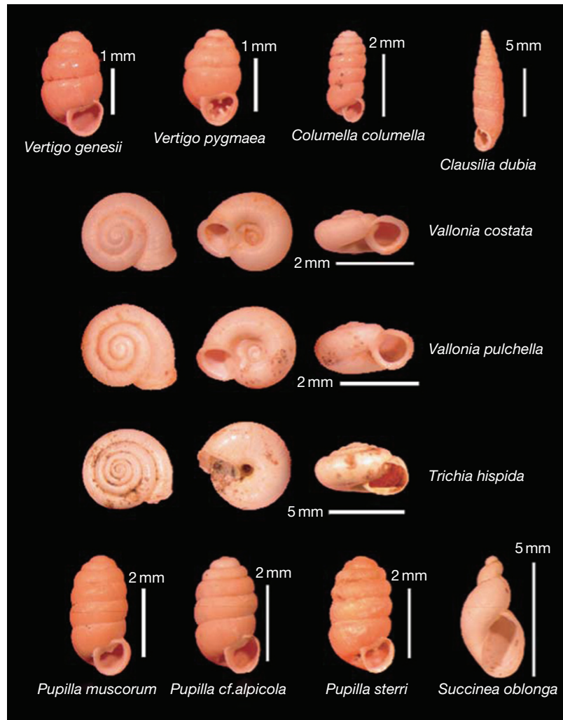
Figure 10 Main terrestrial mollusk species described from loess deposits. Photos by O. Moine.
