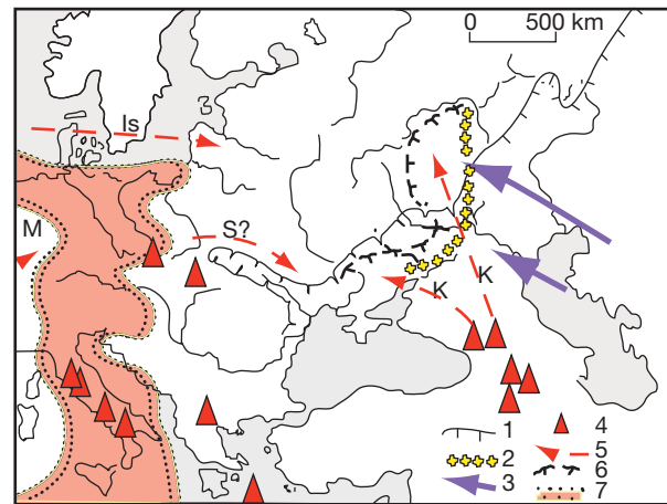
Figure 2 Reach of dust of various origins transported by long-distance eolian transport in eastern and central Europe. Key to symbols: 1, northwesterly extent of western Asiatic dust storms; 2, border between Atlantic and western Asian systems; 3, recorded transport paths of salts; 4, volcanoes active in the Quaternary; 5, volcanic dust pathways (K, north Caucasian; Is, Iceland; S, Sudetic (assumed); M, from Rhine maars); 6, approximate extent of Caucasian volcanic ash; 7, approximate margin of red dust precipitation from the northern Sahara. Reproduced from Rozycki SZ (1991) Loess and Loess-Like Deposits , p. 187. Wrocław: Ossolineum-Polish Academy of Sciences.
