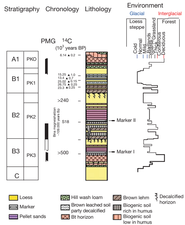
Figure 7 Pedostratigraphy of eastern Europe. Reproduced from Kukla G (1977) Pleistocene land-sea correlations. 1: Europe. Earth-Science Reviews 13: 307–374; Rousseau DD (2001) Loess biostratigraphy: New advances and approaches in mollusk studies. Earth-Science Reviews 54(1–3): 157–171.
