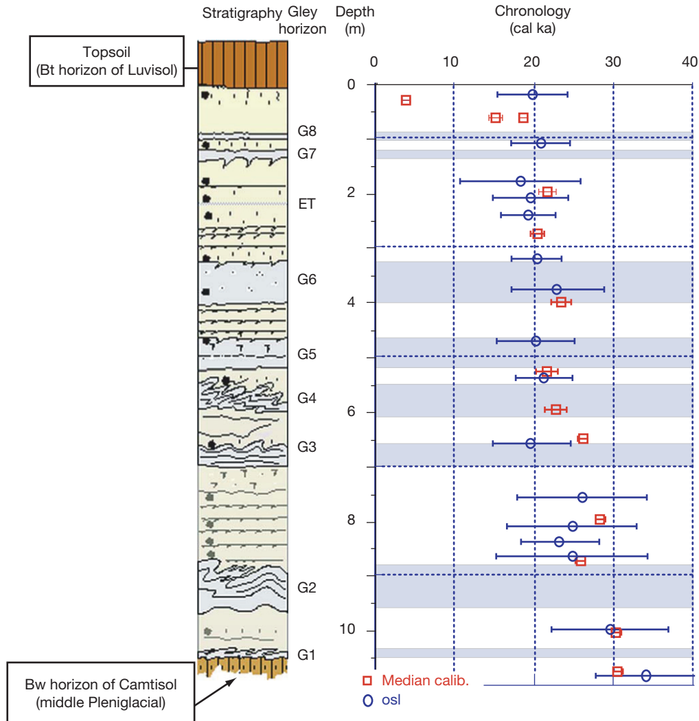
Figure 4 Comparison between the OSL and ^{14}\text{C} dates in the upper Pleniglacial sequence of Nussloch. Key to symbols: G, gley horizon; ET, Eltville Tuff. Data from Hatté et al. (2001a) and Lang et al. (2003).
