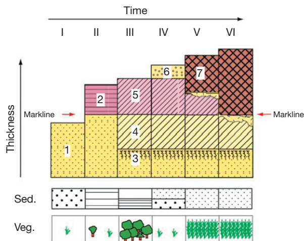
Figure 3 Schematic development of soil complex in loess areas. Reproduced from Kukla G and Koci A (1972) End of the Last Interglacial in the loess record. Quaternary Research 2: 374–383.
