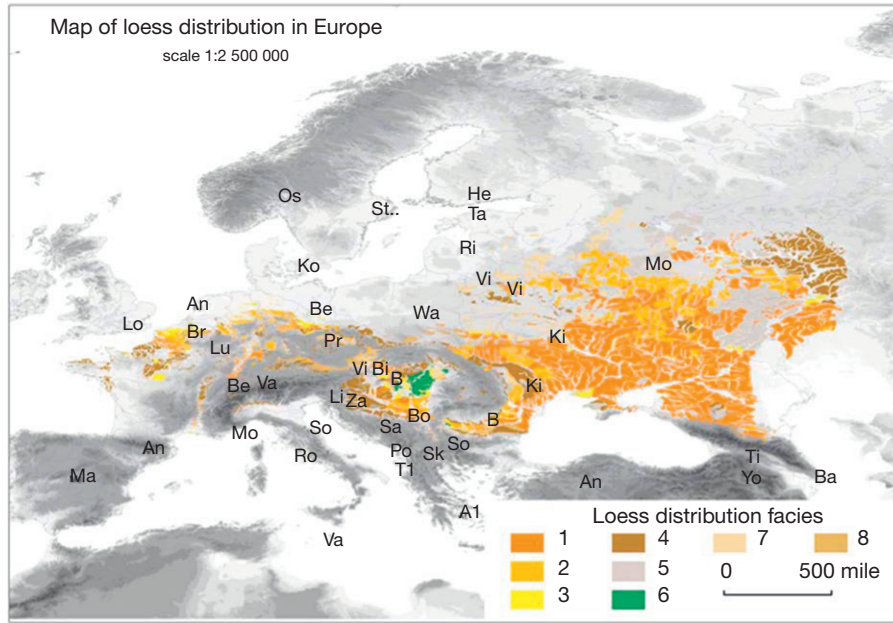
Figure 1 Loess distribution in Europe. Key to symbols: 1, loess >5 m; 2, loess >2 m; 3, sandy loess; 4, loess derivatives; 5, loess and loess derivatives in fragmentary distribution; 6, alluvial loess; 7, eolian sands; 8, loess thickness not differentiated. Reproduced from Haase G, Haase D, Ruske R, Jäger KD, and Altermann M (2006) Loess in Europe – Spatial distribution in a scale 1:2,500,000. Quaternary Science Reviews 26: 1301–1312.
