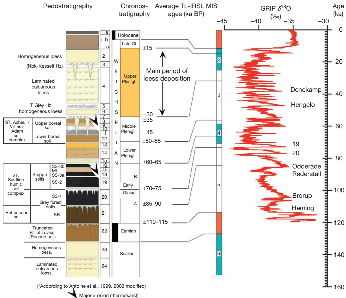
Figure 5 Pedostratigraphy of the upper Pleistocene in western Europe. Reproduced from Antoine P, Rousseau DD, Lautridou JP, and Hatté C (1999) Last interglacial–glacial climatic cycle in loess–paleosol successions of north-western France. Boreas 28: 551–563.
