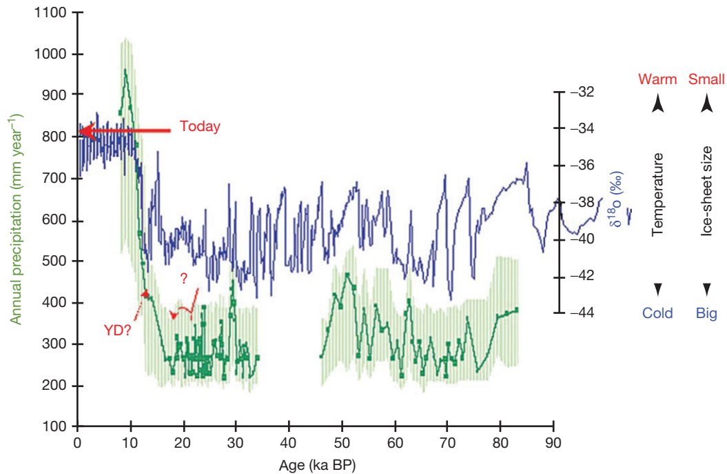
Figure 8 Reconstruction of annual precipitation in the Nussloch sequence. Reproduced from Hatté C and Guiot J (2005) Paleoprecipitation reconstruction by inverse modelling using the isotopic signal of loess organic matter: Application to the Nussloch loess sequence (Rhine Valley, Germany). Climate Dynamics 25: 315–327.
