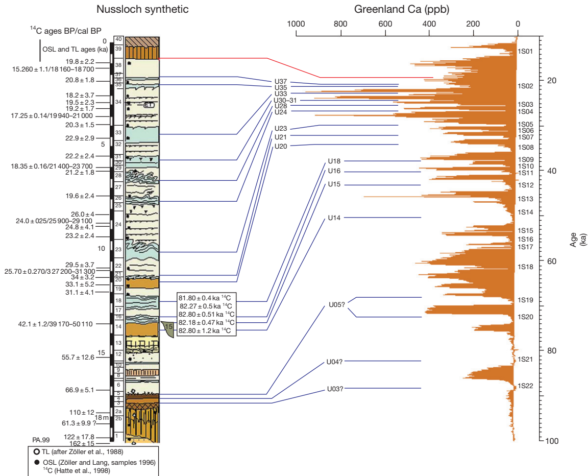
Figure 12 Pedostratigraphy of the Nussloch sequence compared with the Greenland dust record. Reproduced from Antoine P, et al. (2001) High-resolution record of the last interglacial–glacial cycle in the loess paleosol sequences of Nussloch (Rhine Valley–Germany). Quaternary International 76/77: 211–229; Rousseau DD, Antoine P, Hatté C, and Moine O (2003) Enregistrements des événements rapides de type Dansgaard–Oeschger dans les séquences loessiques européennes. Lettre pigb-pmrc-France 15: 21–24.
